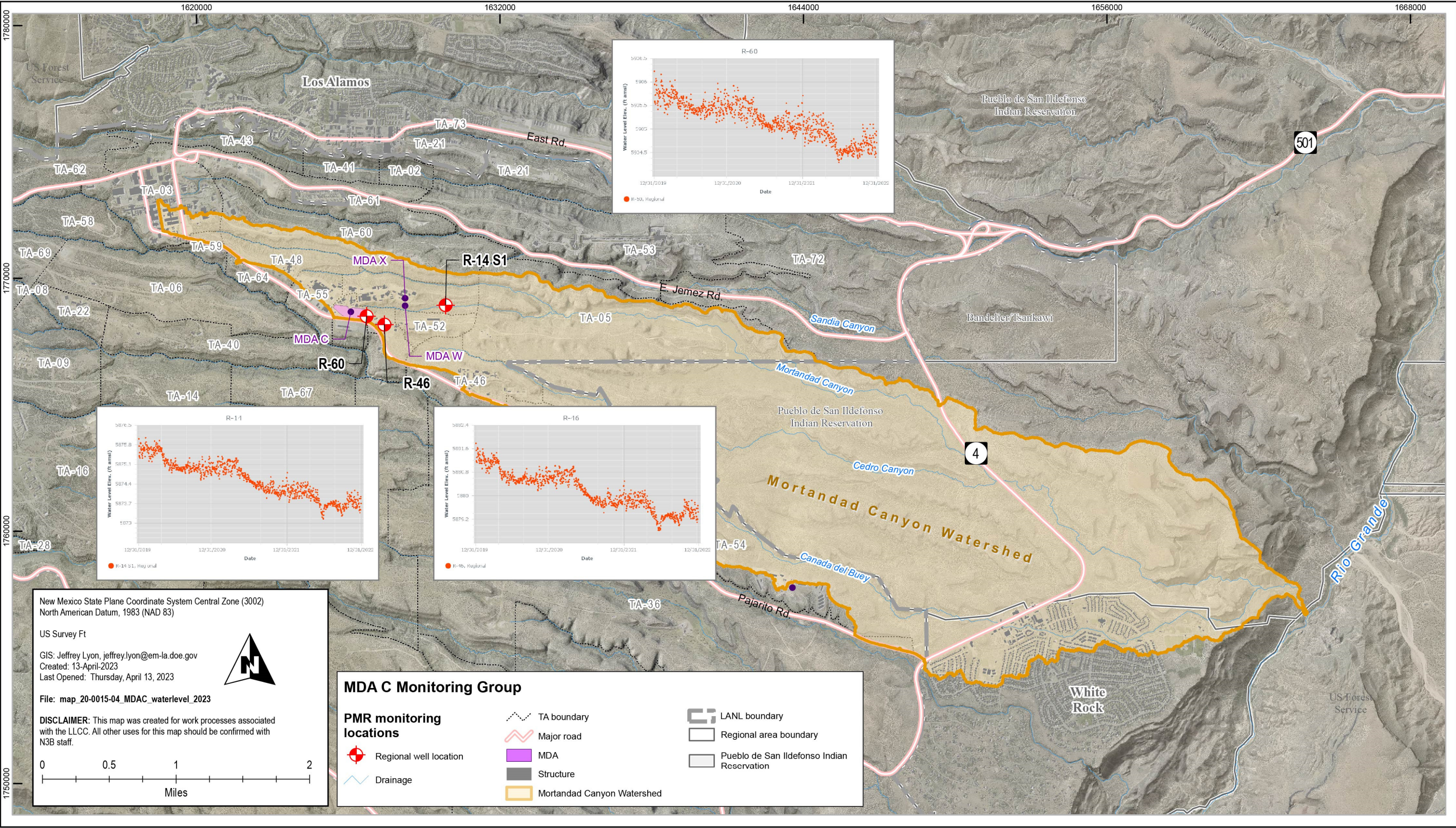
Figure 4.4-1 Groundwater elevations
