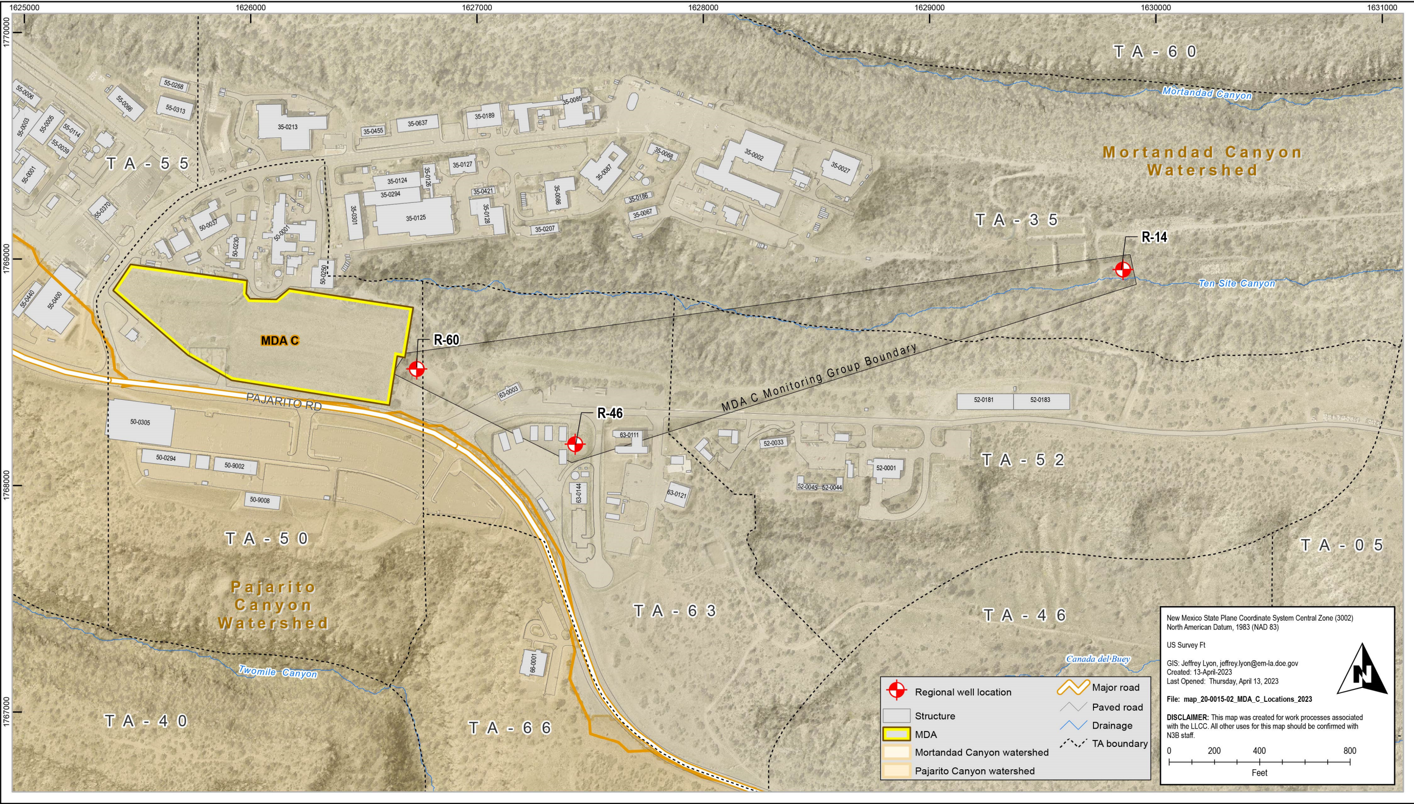
Figure 1.1-2 MDA C monitoring group well locations
