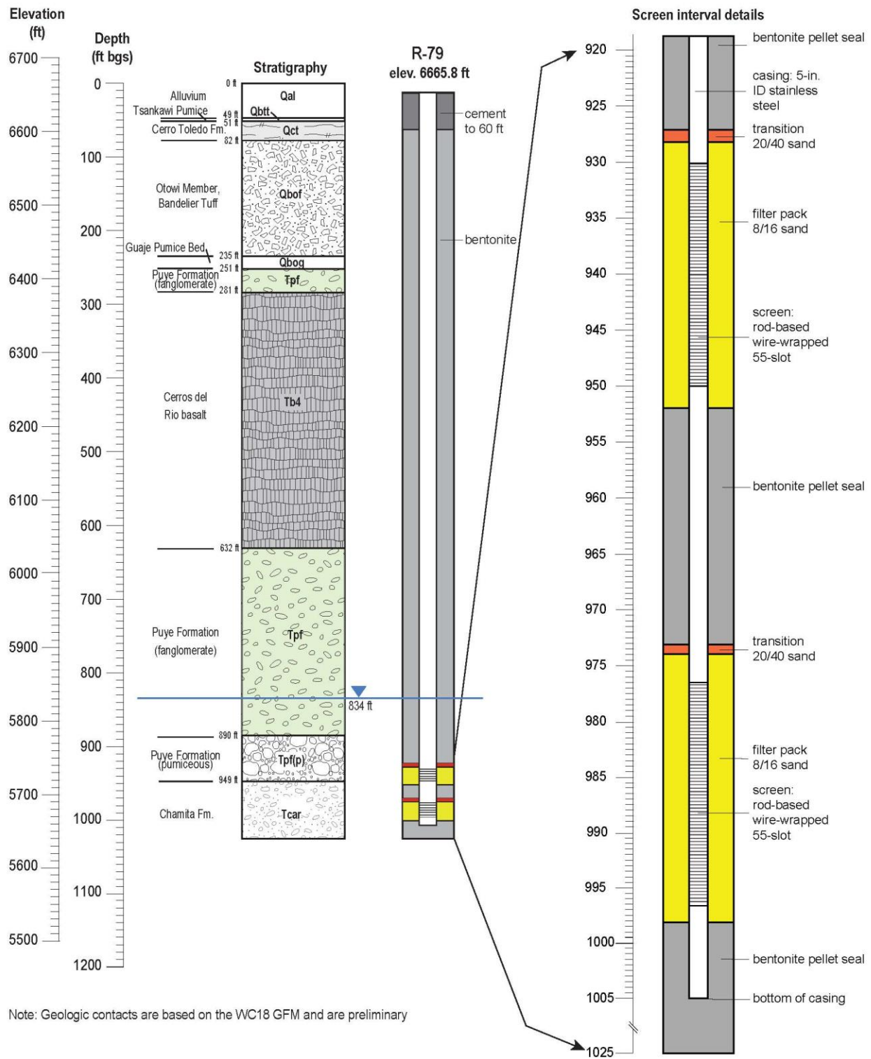
Figure 3 Conceptual well design for R-79
