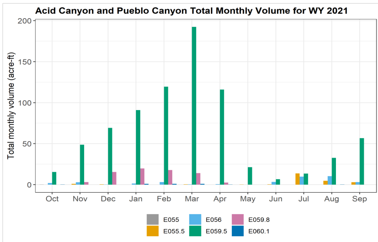
Figure 3 The total monthly volume (acre-ft) for WY 2021 for Acid Canyon and Pueblo Canyon
