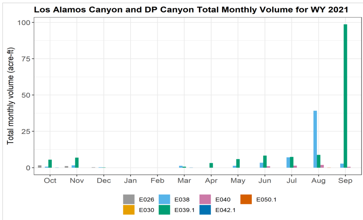
Figure 2 The total monthly volume (acre-ft) for WY 2021 for Los Alamos Canyon and DP Canyon
