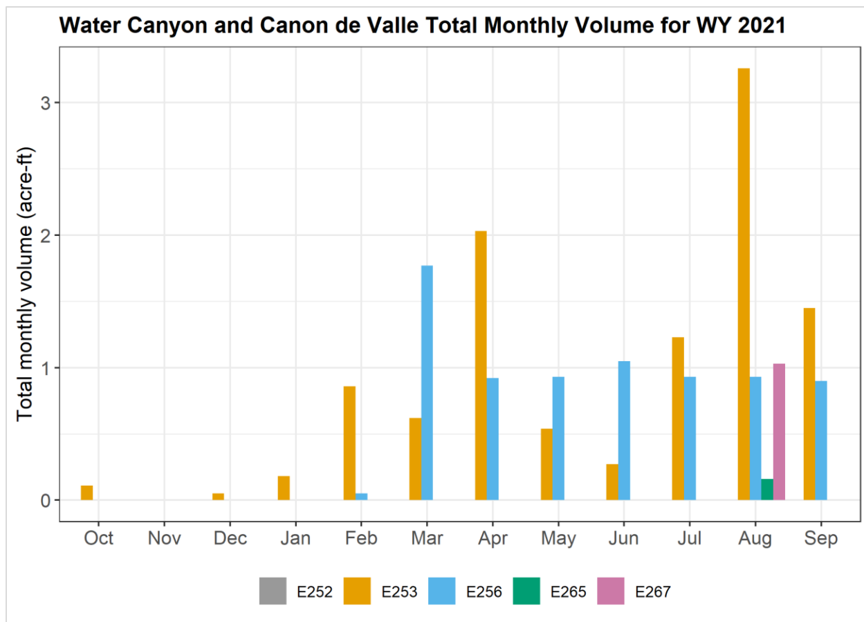
Figure 7 Total monthly volume (acre-ft) for WY 2021 in Water Canyon, Cañon de Valle, and Fence Canyon
