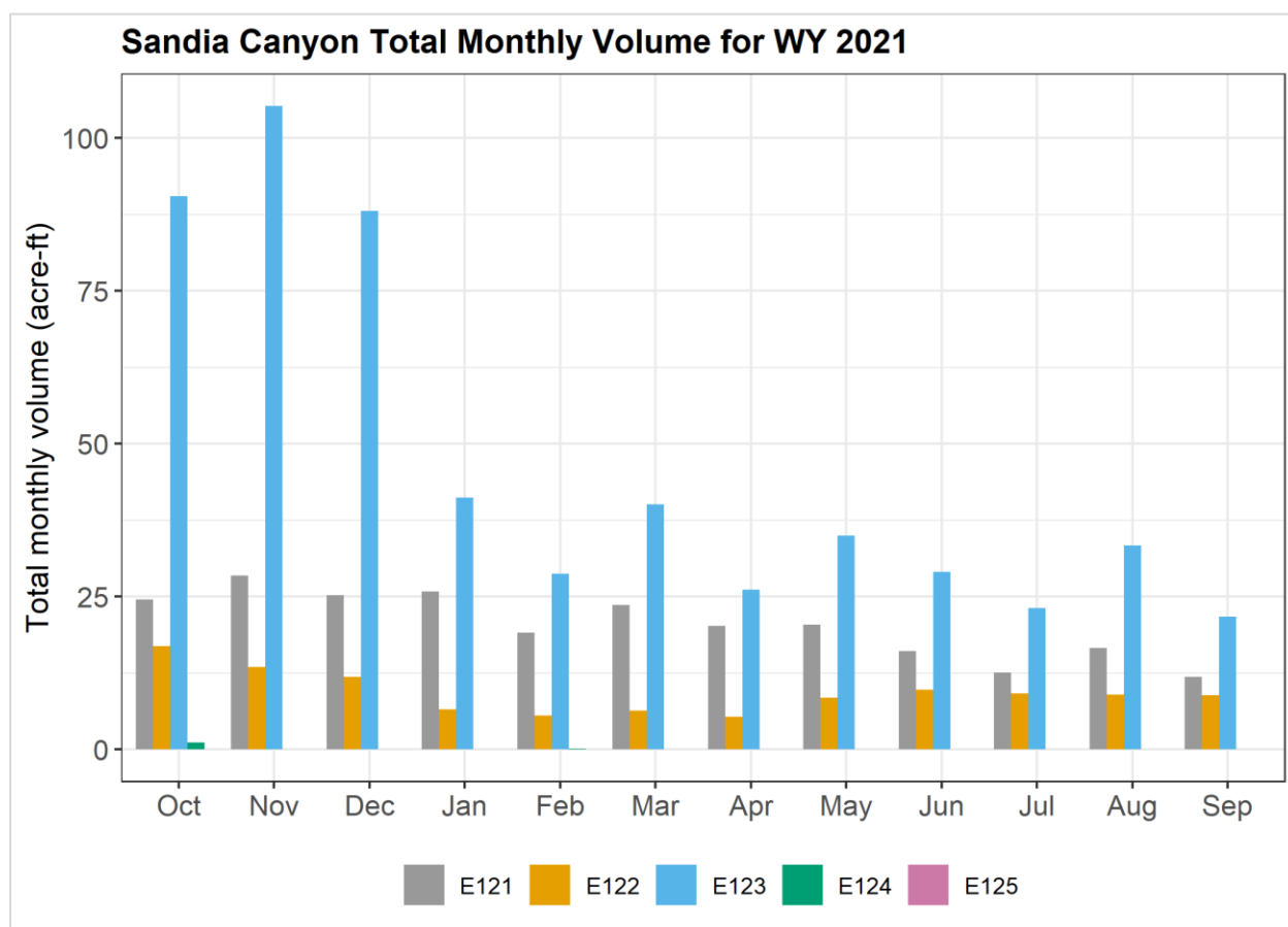
Figure 4 The total monthly volume (acre-ft) for WY 2021 for Sandia Canyon
