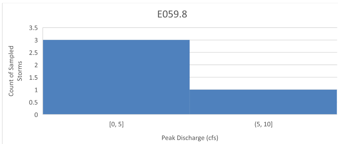
Figure 4.2-1 (continued) Sampled storm event peak discharge distribution 2010–2019
