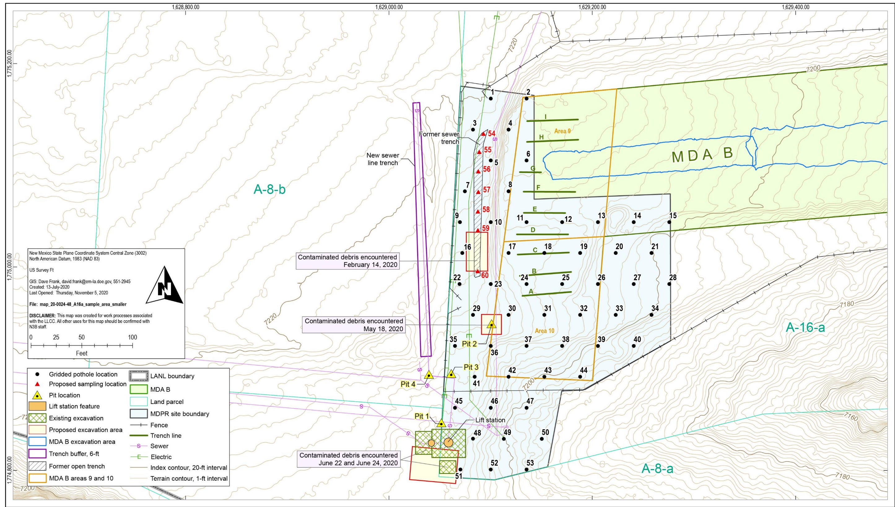
Figure 4.2-2 Proposed potholing locations and excavation areas at Tract A-16-a
