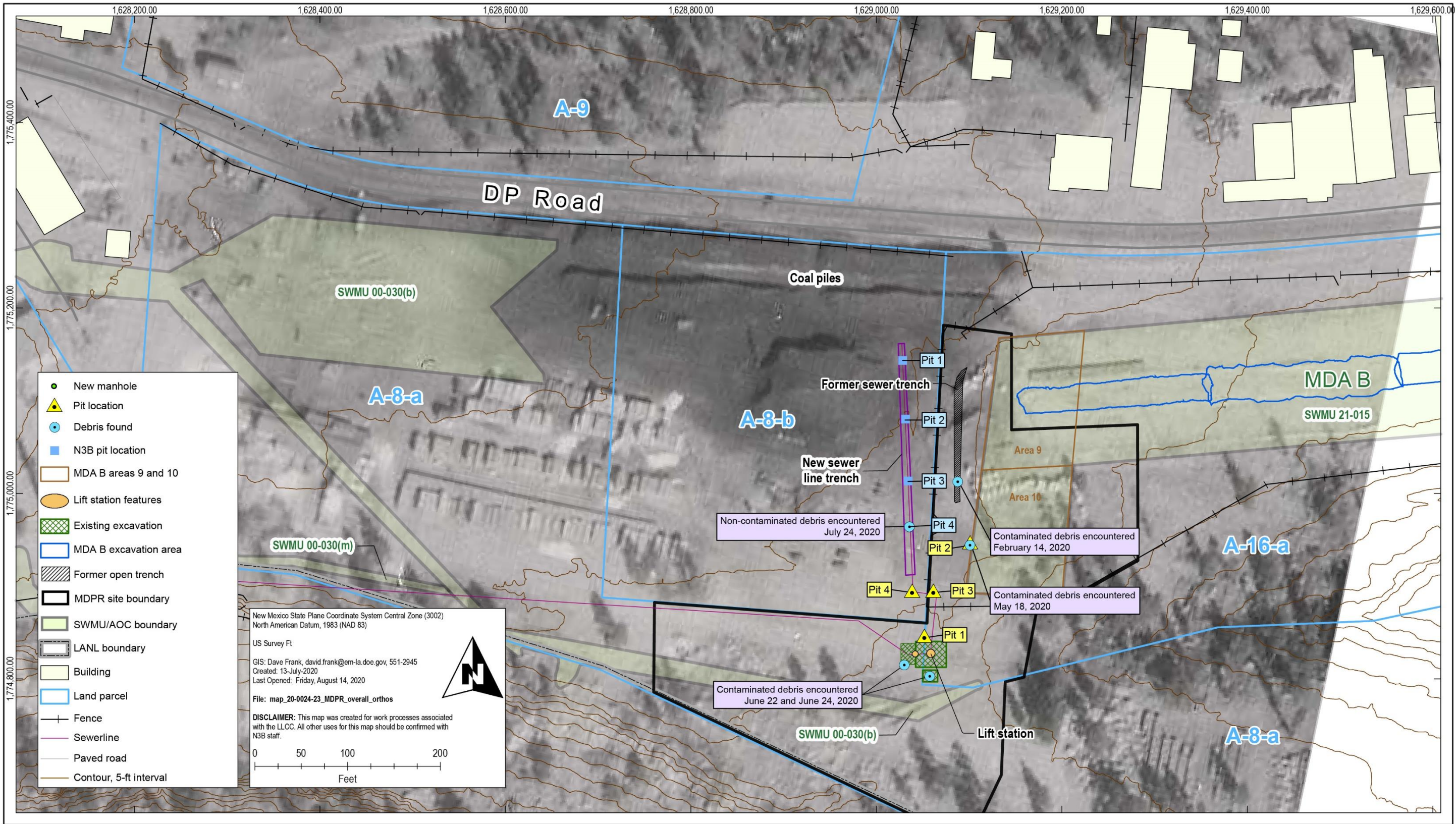
Figure 2.4-4 Overlay of an aerial photograph taken in December 1946 showing the coal piles in relationship to Tracts A-8-b and A-16-a and MDPR site features
