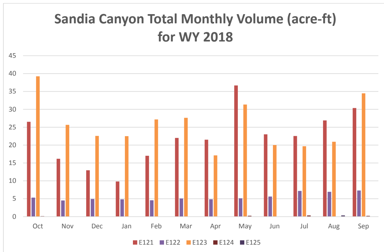
Figure 6 The total monthly volume (acre-ft) for WY 2018 for Sandia Canyon
