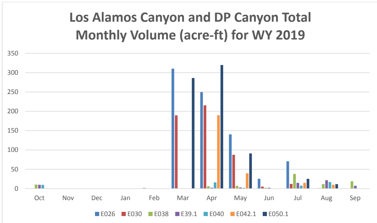
Figure 3 The total monthly volume (acre-ft) for WY 2019 for Los Alamos Canyon and DP Canyon
