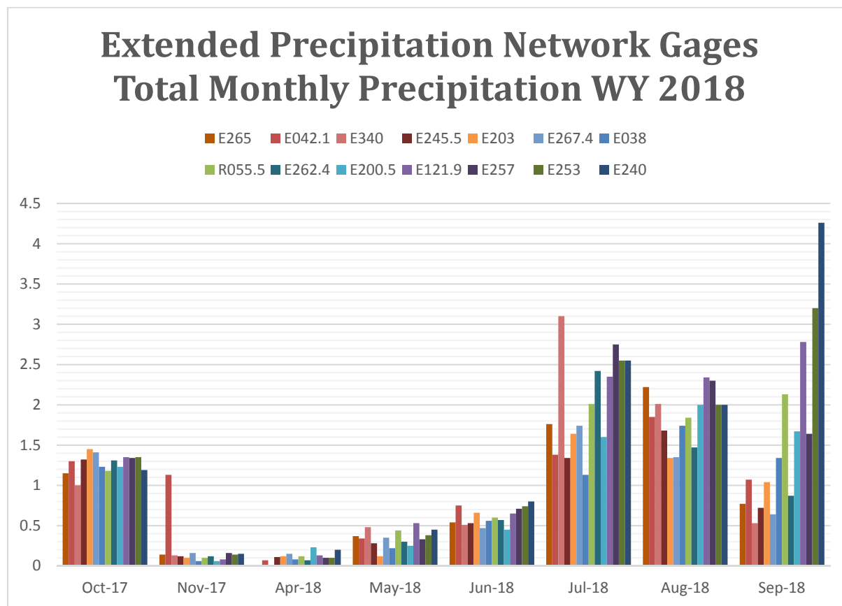
Figure 16 Total monthly precipitation for the extended precipitation network gages for WY 2018, excluding December 2017 to March 2018, when the gages were shut down for winter
