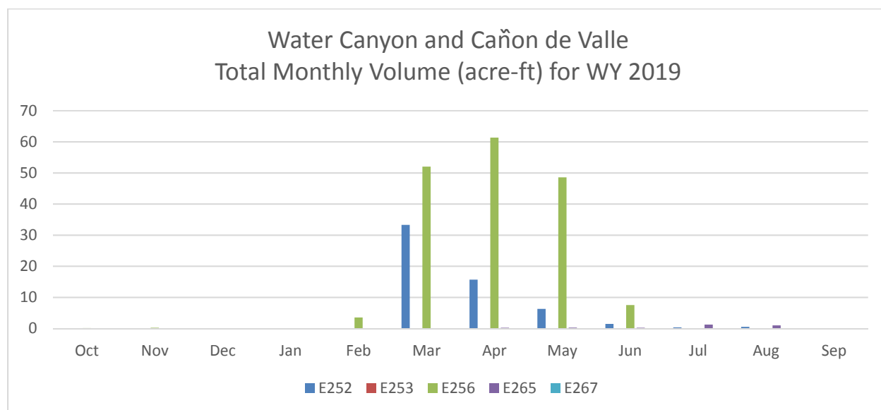
Figure 13 Total monthly volume (acre-ft) for WY 2019 in Water Canyon, Cañon de Valle, and Fence Canyon
