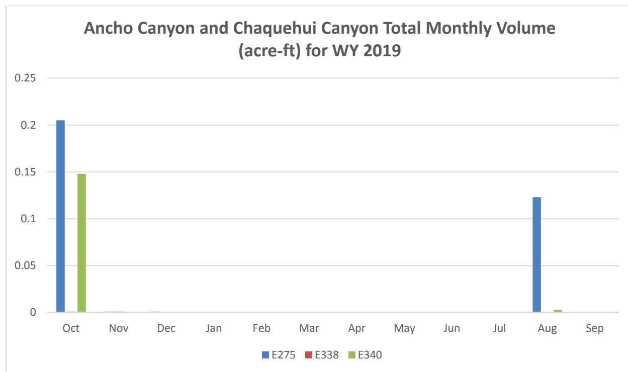
Figure 15 Total monthly volume (acre-ft) for WY 2019 in Ancho Canyon and Chaquehui Canyon
