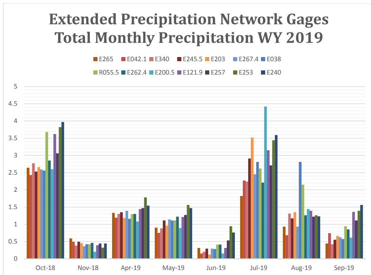
Figure 17 Total monthly precipitation for the extended precipitation network gages for WY 2019, excluding December 2018 to March 2019, when the gages were shut down for winter
