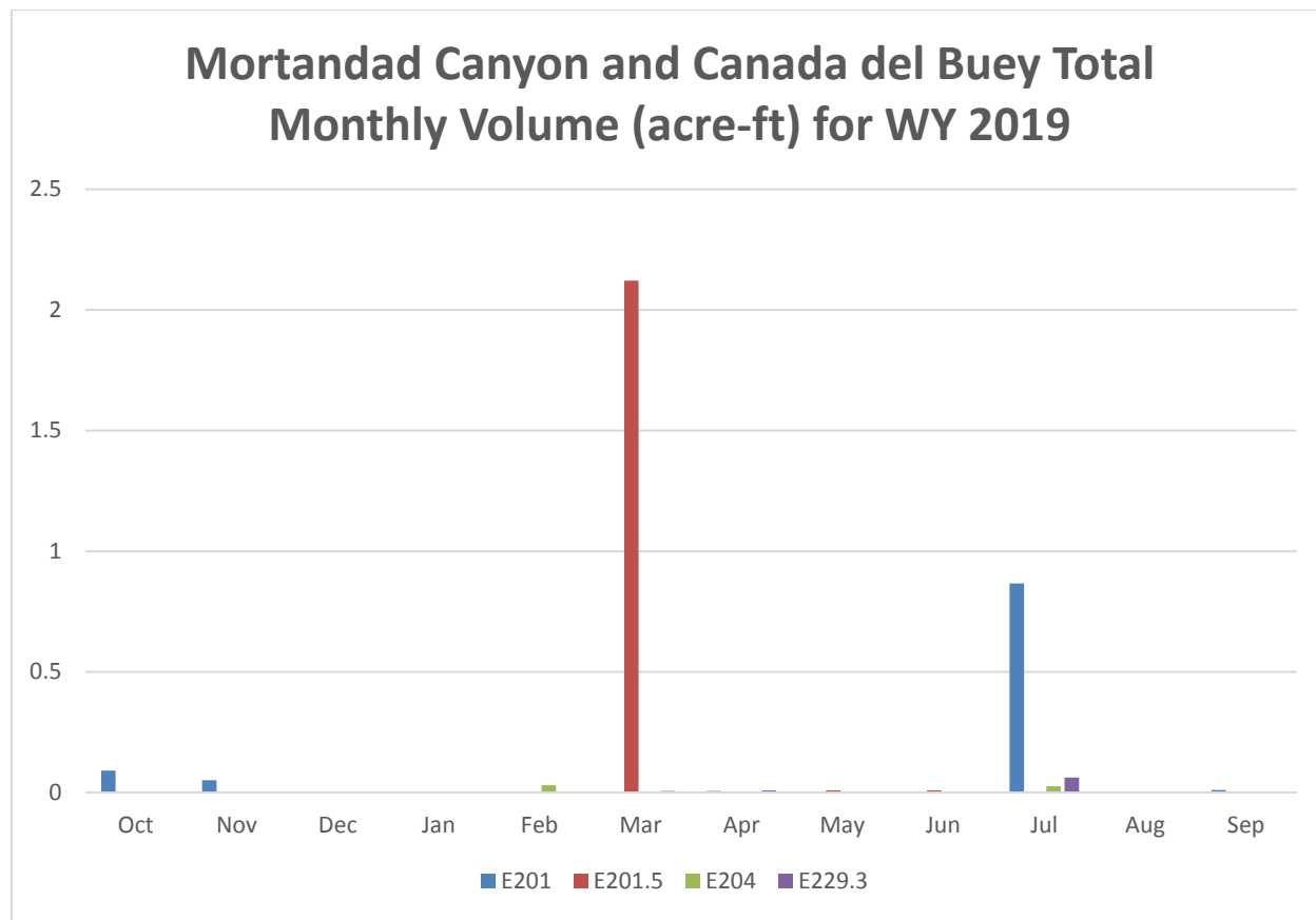
Figure 9 Total monthly volume (acre-ft) for WY 2019 in Mortandad Canyon and Cañada del Buey
