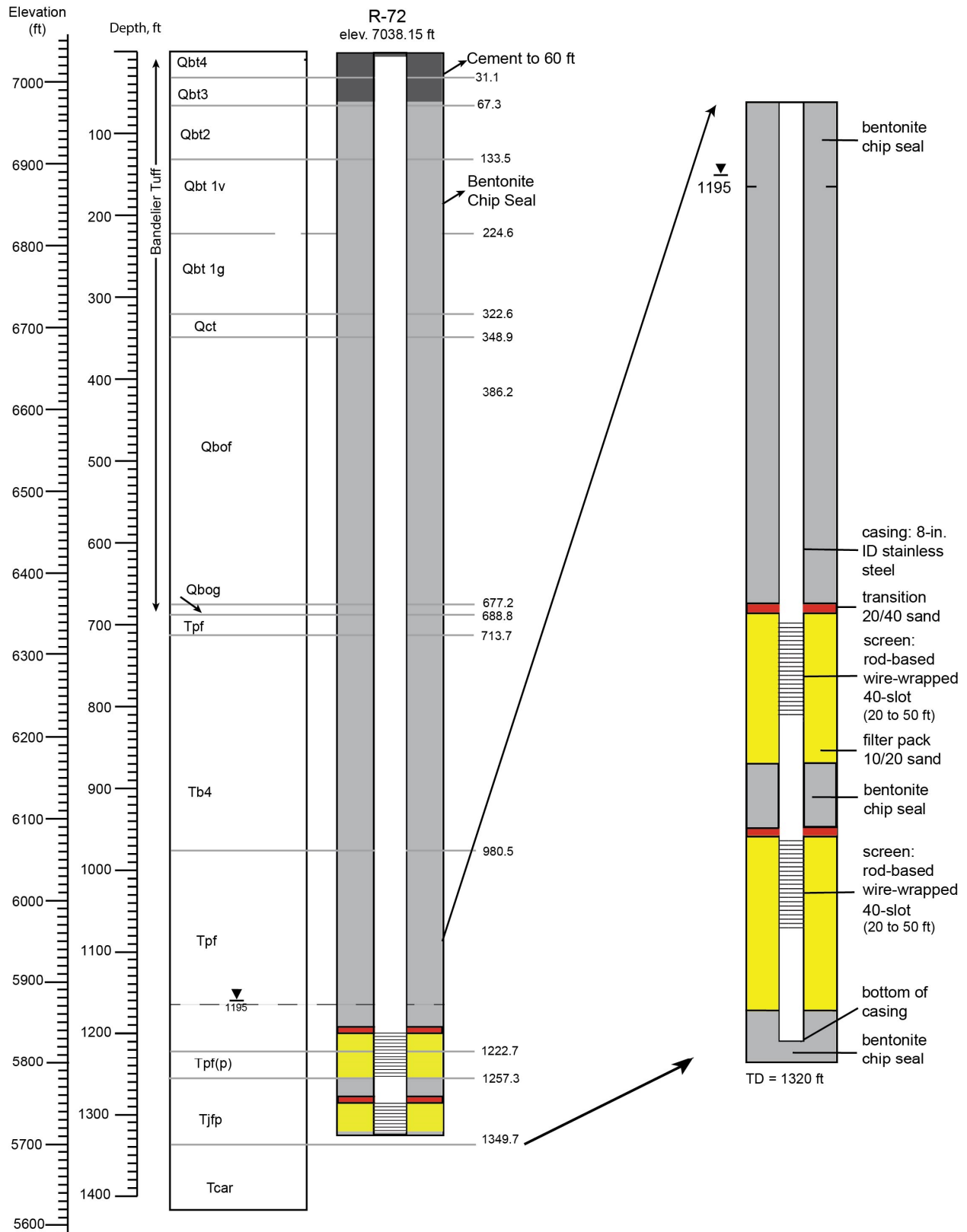
Figure 3 R-72 conceptual well design
